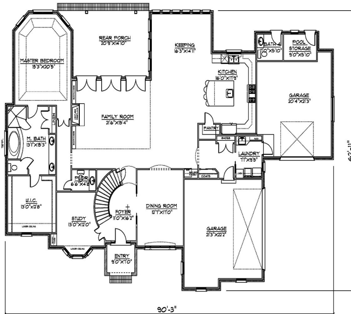
FLOOR PLAN FIRST FLOOR
