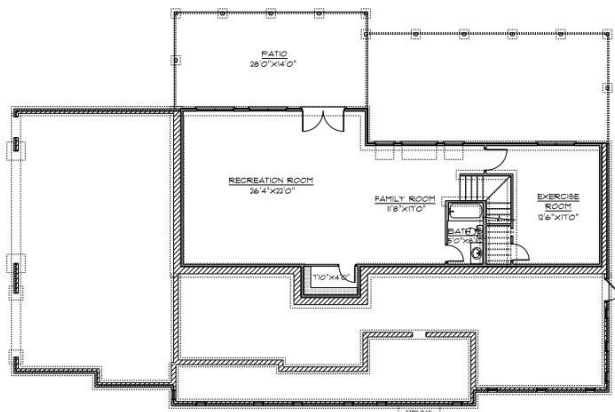
BASEMENT PLAN
