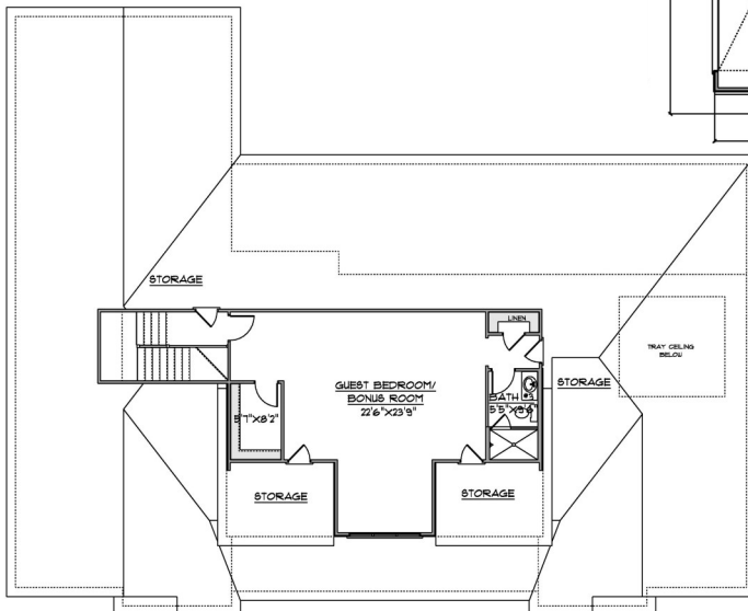
FLOOR PLAN SECOND FLOOR
