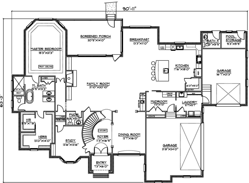
FLOOR PLAN FIRST FLOOR
