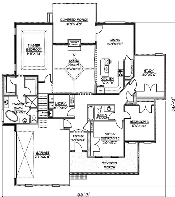
FLOOR PLAN FIRST FLOOR
