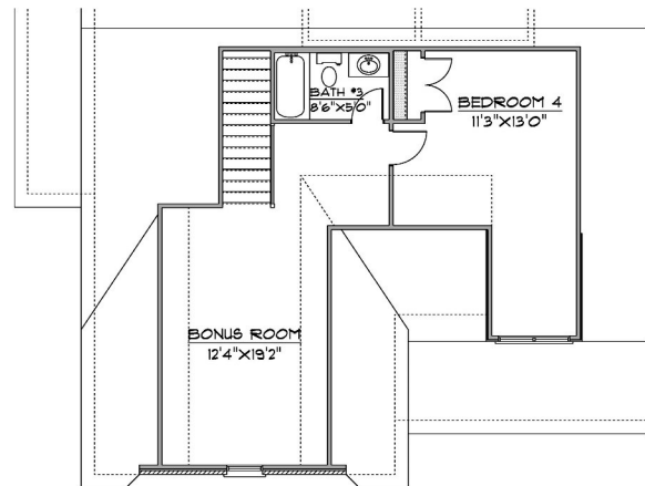
FLOOR PLAN SECOND FLOOR
