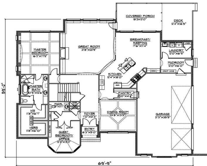
FLOOR PLAN 1ST FLOOR
