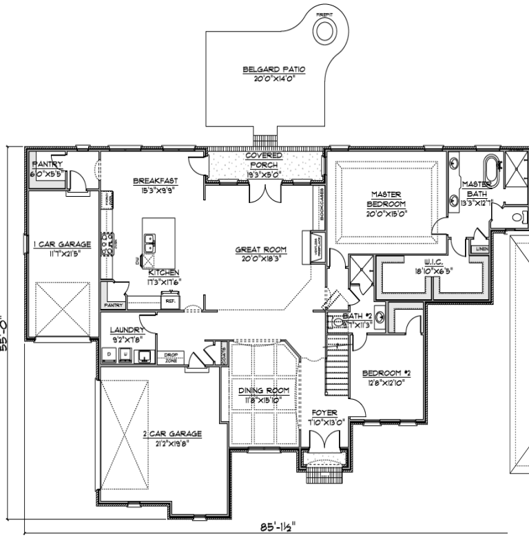
FLOOR PLAN FIRST FLOOR
