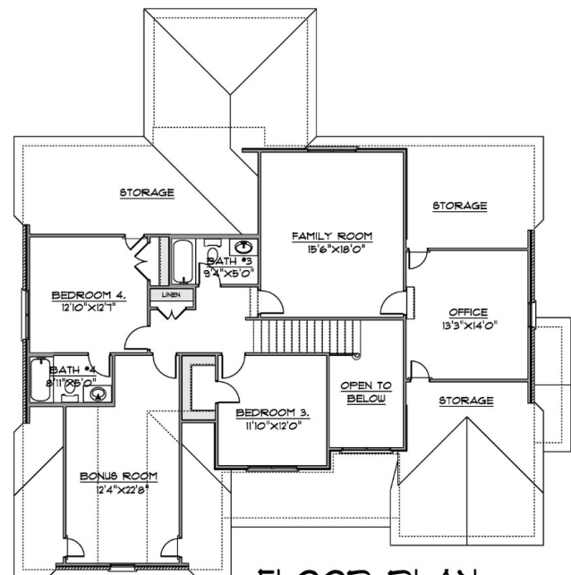
FLOOR PLAN SECOND FLOOR
