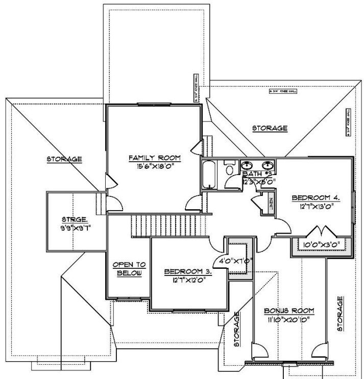
FLOOR PLAN SECOND FLOOR
