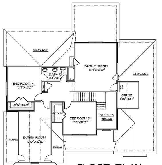
FLOOR PLAN SECOND FLOOR
