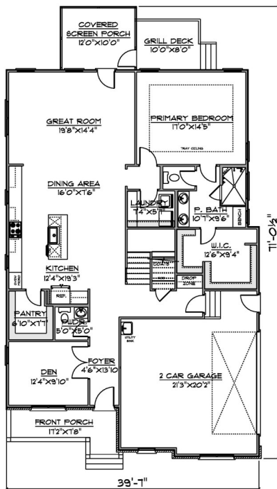
FLOOR PLAN FIRST FLOOR
