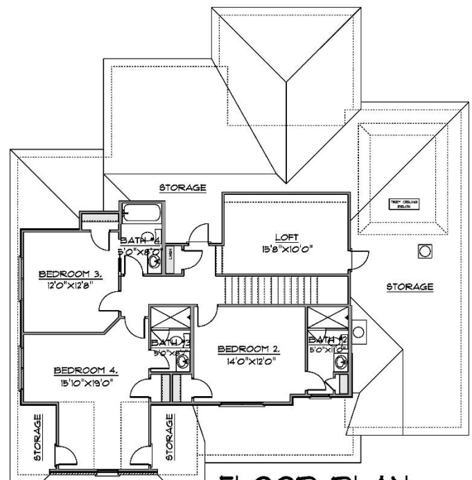
FLOOR PLAN SECOND FLOOR
