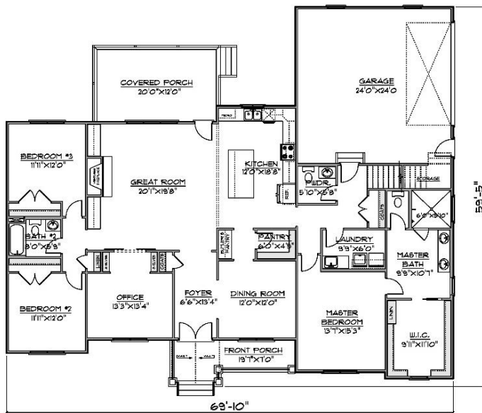
FLOOR PLAN FIRST FLOOR
