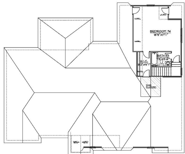
FLOOR PLAN SECOND FLOOR
