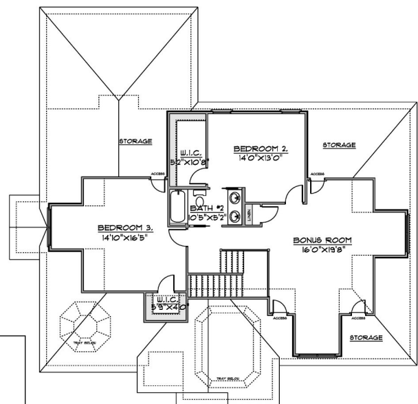
FLOOR PLAN SECOND FLOOR
