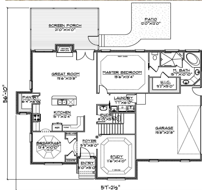
FLOOR PLAN FIRST FLOOR
