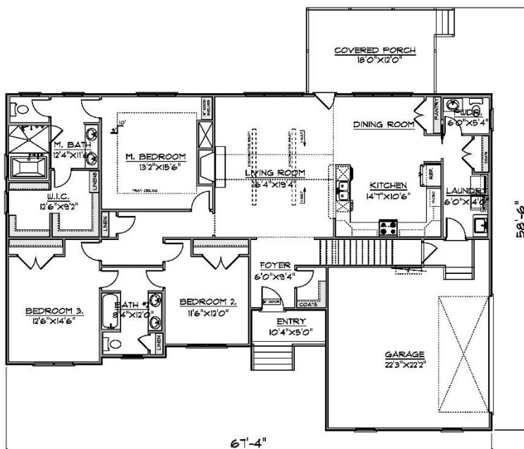
FLOOR PLAN FIRST FLOOR
