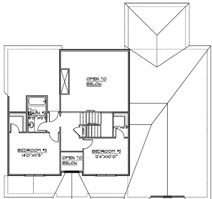
FLOOR PLAN SECOND FLOOR
