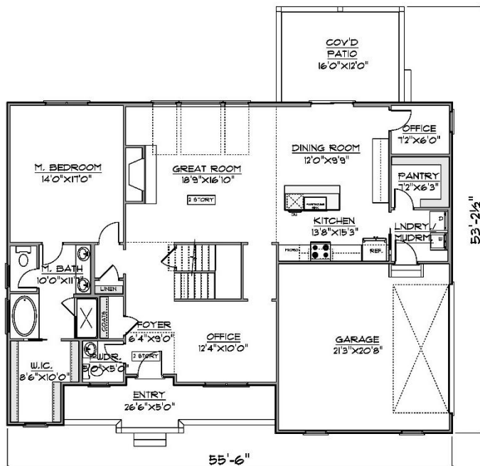
FLOOR PLAN FIRST FLOOR
