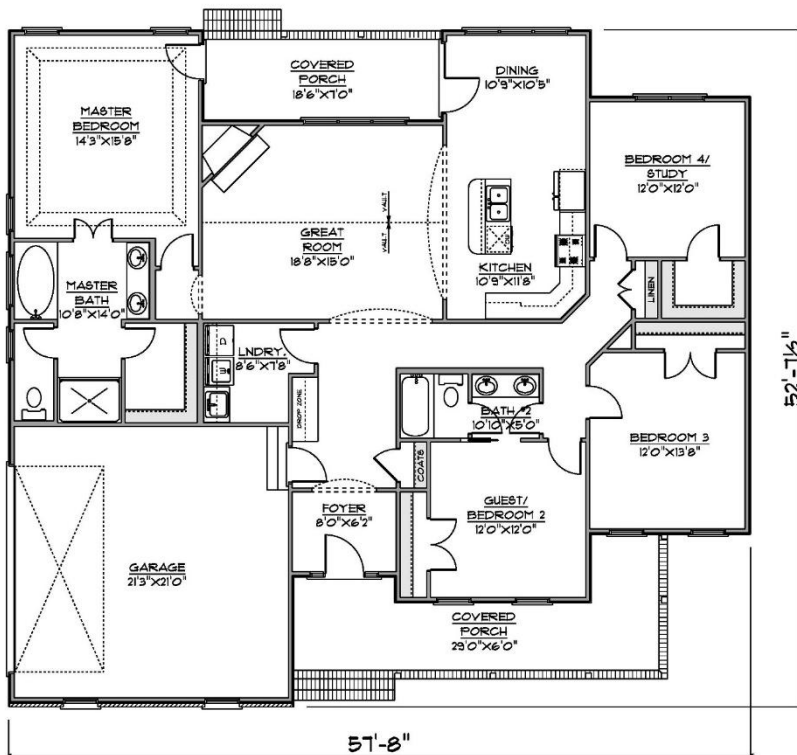
FLOOR PLAN FIRST FLOOR
